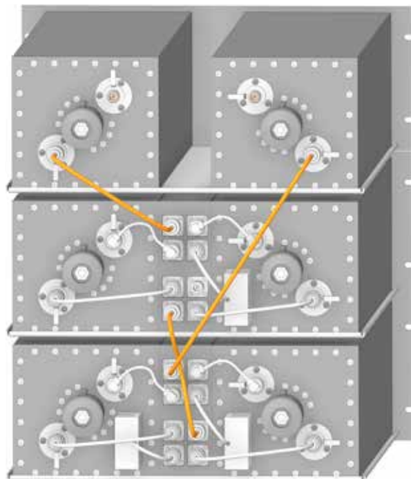
MCPD180-V/2-2 F06VR180M2DDxxxx
